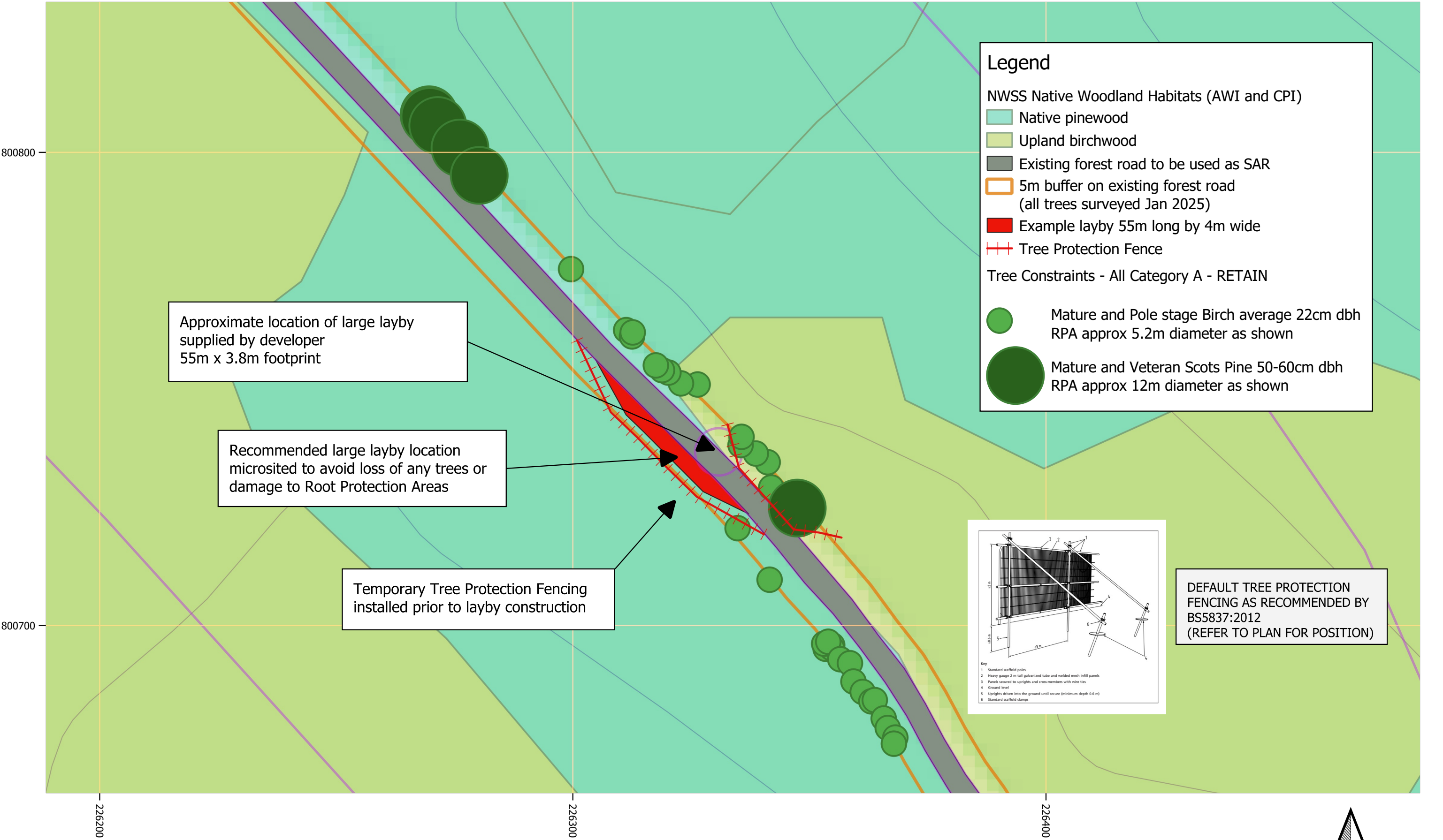
Appendix 9.2 Figure 1: Example Tree Protection Plan (to BS:5837) for SAR large layby location
