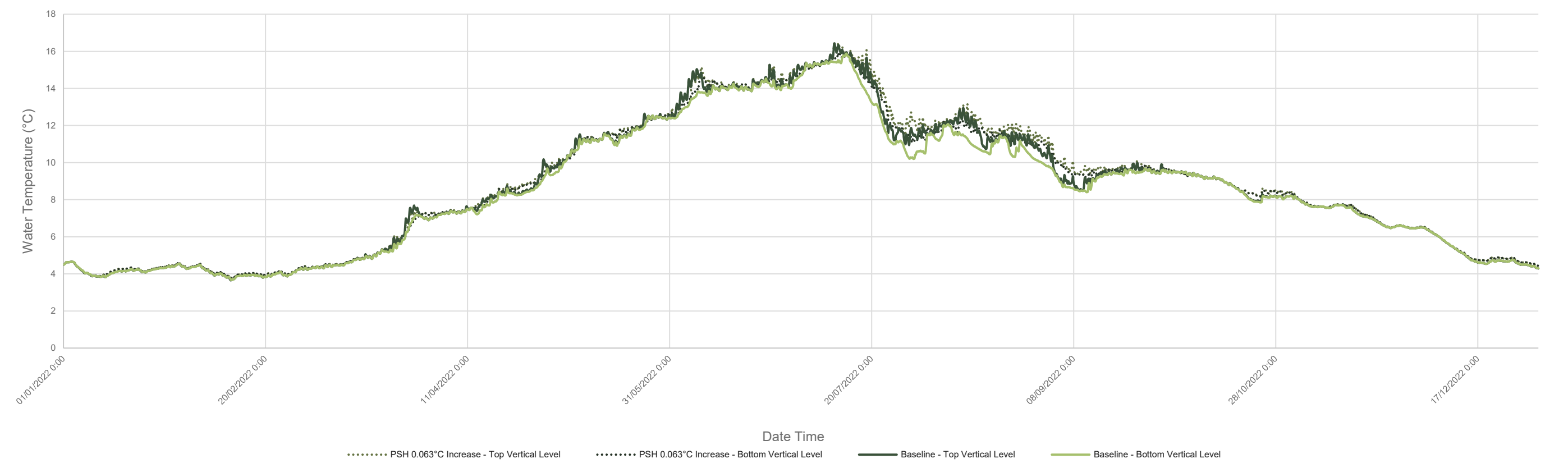
Figure 3-25: Vertical Temperature Profile at Dam Outtake (PSH 0.063°C Increase)
