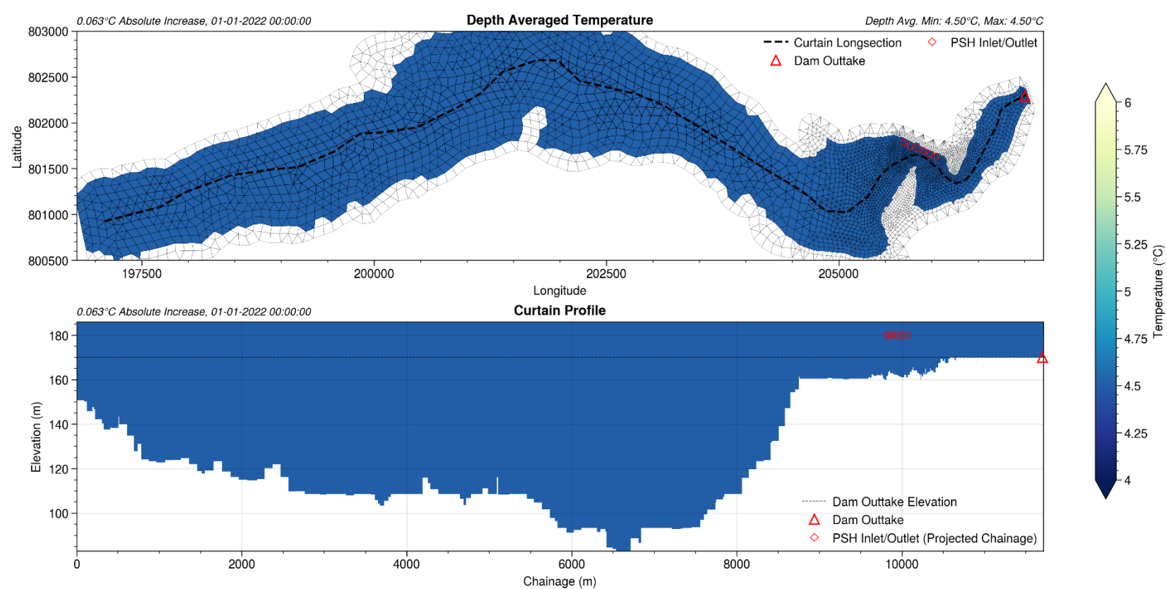
Figure 3-15: Curtain Plot of Temperature Profile Along Longitudinal Trace (PSH 0.063°C Increase at time 01/01/2022 00:00:00)
