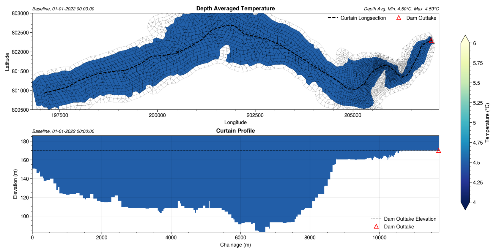
Figure 3-9: Curtain Plot of Temperature Profile Along Longitudinal Trace (Baseline 2022 at time 01/01/2022 00:00:00)
