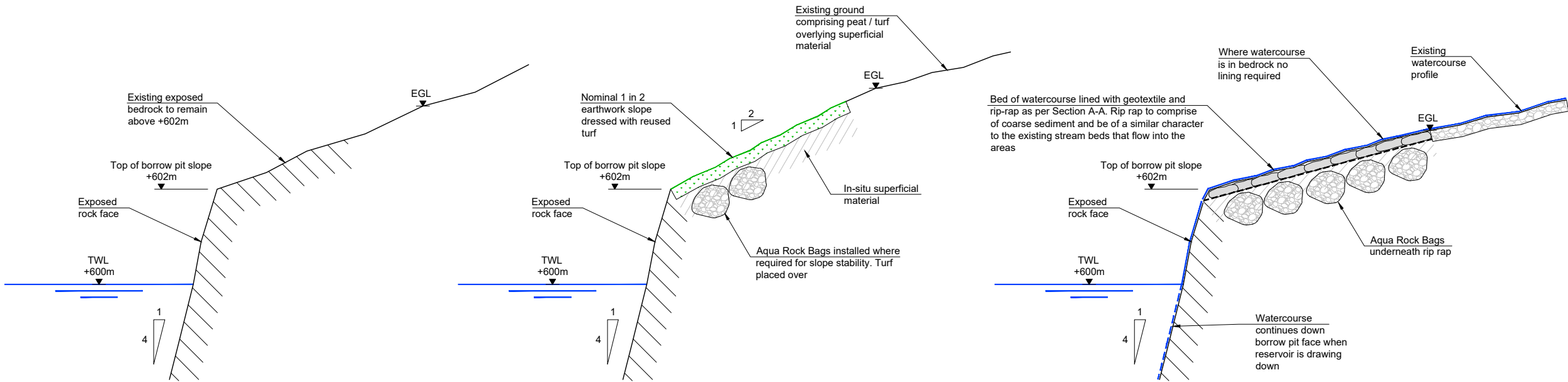
Typical Shoreline Section - Bedrock Areas 1:100 @ A3
