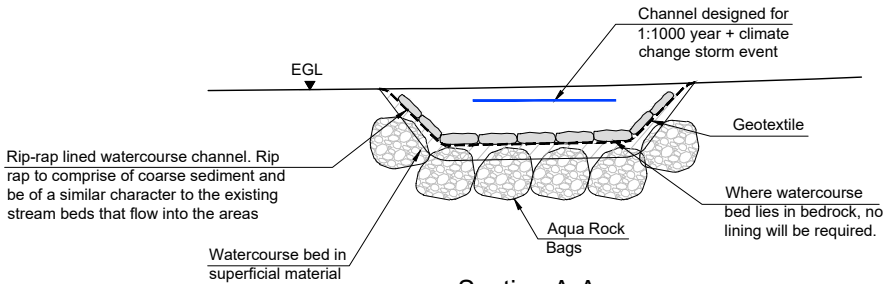
Section A-A Reinforced Bed In Superficial Material 1:100 @ A3
